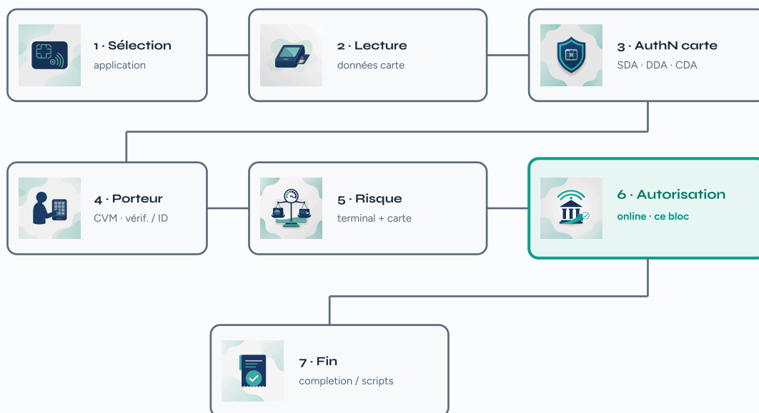
Cycle de vie transaction EMV
